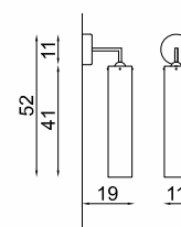
M160/A1 H 52 cm - Sp 19 cm L 11 cm E27 1x60W Max
